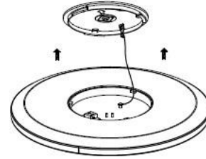
2. One end of the safety rope is stuck at the top plate hook, and one end is buckled at the lamp body hook to ensure that the installation is reliable
