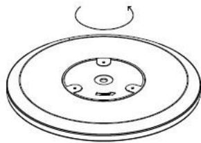
5. The AC line is pierced from the top disc round hole, and the top disc arrow is aligned and rotated clockwise to a "click" sound, which is installed in place
